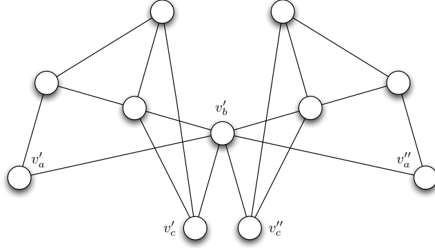
Figure 1: The graph \tilde{\mathcal{G}}
