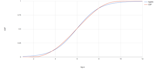
Figure 3: Logistic fit of empirical weight distribution
