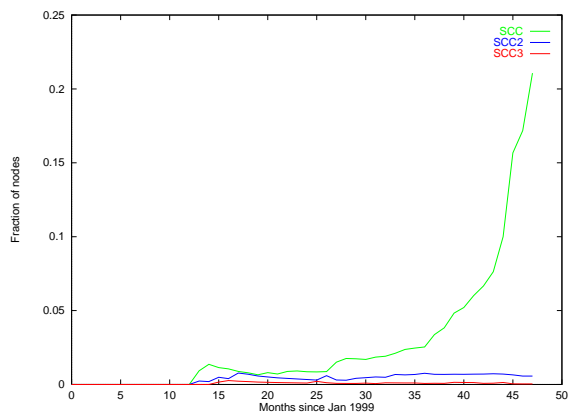
Figure 3: SCC evolution
