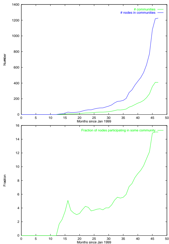
Figure 4: Community evolution
