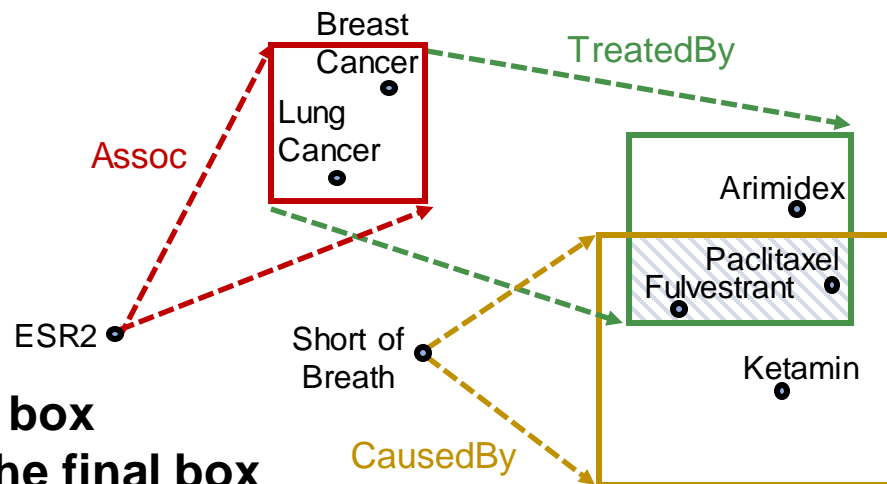
Embedding Space
