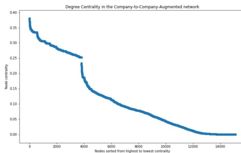
Fig. 8: Degree centrality scores in Companies-to-Companies-Augmented
