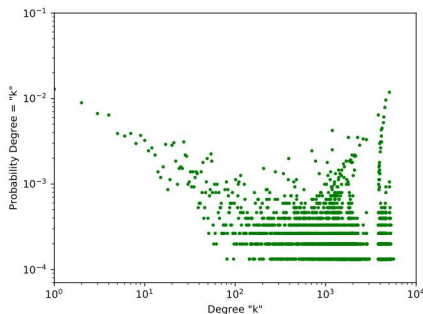
Fig. 5: Degree distribution for Companies-to-Companies-Augmented network.
