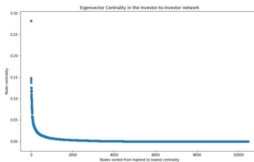
Fig. 9: Eigenvector centralities for nodes in Investors-to-Investors
